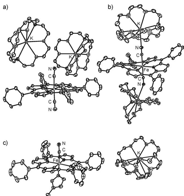
Figure 1. a,b) ORTEPs of two [K(222)] 2 [Fe(tp)(CN) 2 ] structures, showing two different coordination modes: a) [K(222)] 2 [Fe(tp)(CN) 2 ] 4PhCl and b) one of two [K(222)] 2 [Fe(tp)(CN) 2 ] PhCl units. c) The structure of [K(222)][Fe(tp)(CN)(1-Melm)]. All three structures illustrated are at 100 K. Ellipsoids set at 50% probability, hydrogen atoms omitted for clarity.
