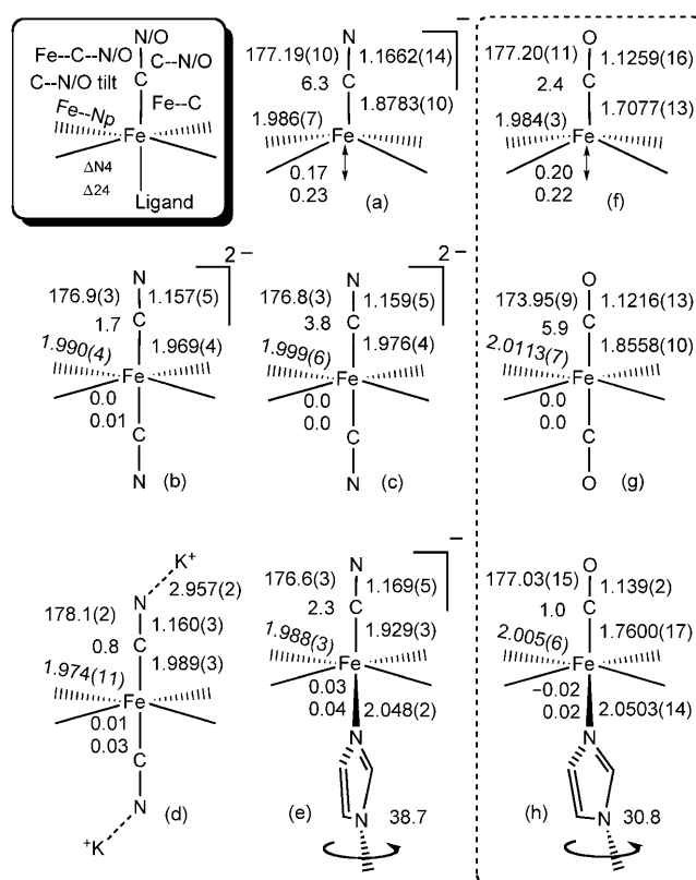
Figure 2. The coordination groups of a) [K(222)][Fe(tp)(CN)] (polymorph 1), b) [K(222)] 2 [Fe(tp)(CN) 2 ], c) [K(222)] 2 [Fe(tp)(CN) 2 ], d) [K(222)] 2 [Fe(tp)(CN) 2 ], and e) [K(222)][Fe(tp)(CN)(1-Melm)]. Structures of f) [Fe(oep)CO], [20] g) [Fe(oep)(CO) 2 ], [20] and h) [Fe(tp)CO(1-Melm)] [24] are also shown for comparison. The boxed key (upper left) indicates the structural parameters that are given for each structure. \Delta_{N4} and \Delta_{24} are the iron displacements from the four-nitrogen and 24-atom mean planes. The dihedral angle between the imidazole plane and the closest N p –Fe–N ax fragment is also shown for the imidazole derivatives. All the structures were obtained at 100 K.
